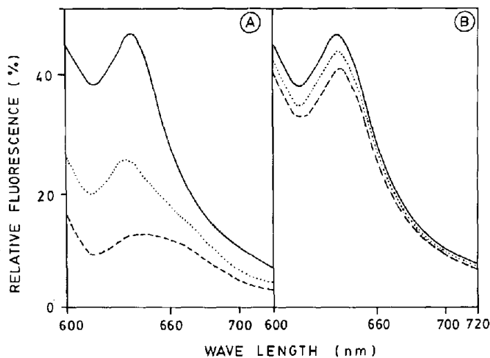
Figure 3. PBS fluorescence emission spectra (600–720 nm) of intact cells of A. flos-aquae were recorded in relative units (%) at room temperature. Cells with equimolar concentrations of \text{Hg}^{2+} (A) and \text{Cd}^{2+} (B) were incubated for 30 min prior to use. The wavelength of excitation was 570 nm. The cells were treated without (—) and with different concentrations of each metal: 10 \mu\text{M} (.....) and 20 \mu\text{M} (---). The concentration of chlorophyll a was kept at 5 \mu\text{g ml}^{-1} .
