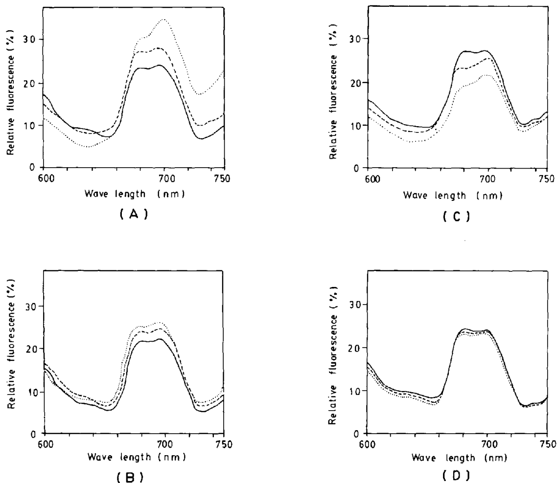
Figure 4. Chlorophyll a fluorescence emission spectra (600–750 nm) of intact cells of A. flos-aquae were recorded in relative units (%) at room temperature (25 °C). The cells were supplemented with \text{Hg}^{2+} alone (A) and \text{Hg}^{2+} plus 100 \mu\text{M} of \text{NH}_2\text{OH} (B), and were light incubated for 30 min. The wavelength of excitation was 435 nm prior to use. The cells were treated without (—) and with different concentrations of \text{Hg}^{2+} : 10 \mu\text{M} (---) and 20 \mu\text{M} (.....). Chlorophyll a fluorescence emission spectra (600–750 nm) of the intact cells of A. flos-aquae were recorded in relative units (%) at room temperature (25 °C) in the presence of \text{Cd}^{2+} alone (A) and \text{Cd}^{2+} plus 100 \mu\text{M} of \text{NH}_2\text{OH} (B). The wavelength of excitation was 435 nm. The cells supplemented without (—) and with 10 \mu\text{M} (---) and 20 \mu\text{M} (.....) of \text{Cd}^{2+} were light incubated for 30 min prior to use.
