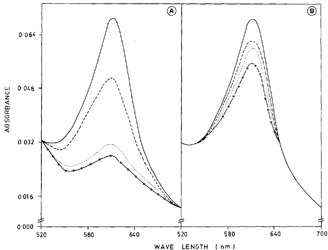
Figure 2. Absorption spectra of the extracted PC pigment in the presence of equimolar concentrations of \text{Hg}^{2+} (A) and \text{Cd}^{2+} (B). The extracted PC was incubated for 5 min without (—) and with different concentrations of each metal: 5 \mu\text{M} (---), 10 \mu\text{M} (.....) and 20 \mu\text{M} (—○—).
